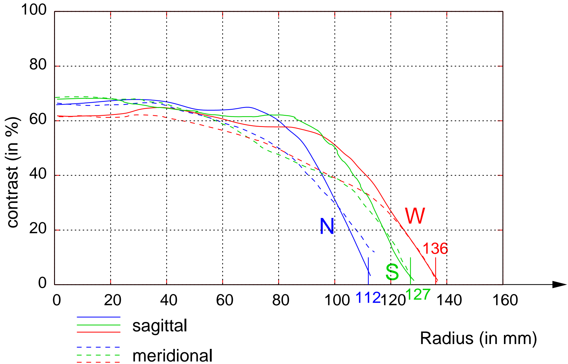
FTM curves @f/22 / @ 20 cy/mm for Apo Sironar N, S et W / focal length = 150 mm
