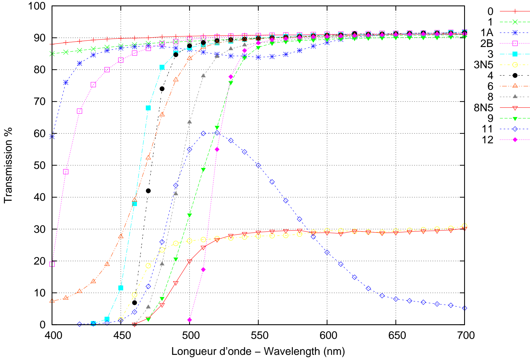
Filtres Wratten® – Transmission – Wratten® filters
