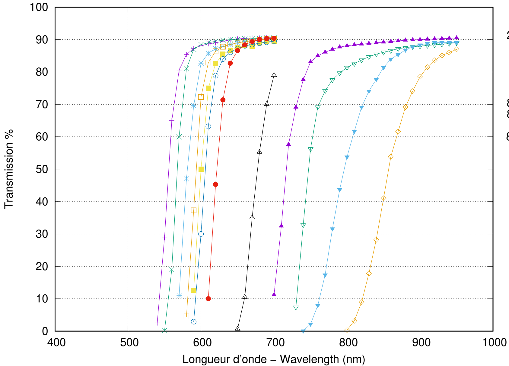
Filtres Wratten® – Transmission – Wratten® filters orange – rouge / red – infra-rouge / infra-red
